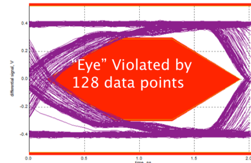
1 st -GEN Device Active EMI Disabled Eye Diagram
