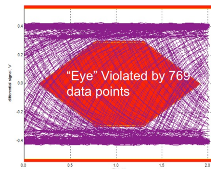
1 st -GEN Device Eye Diagram
